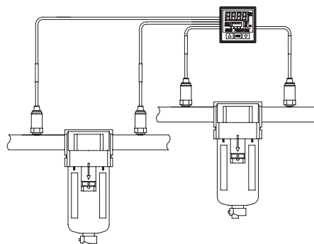
Multi-channel controller for detecting differential pressure PSE201-X101 Series
